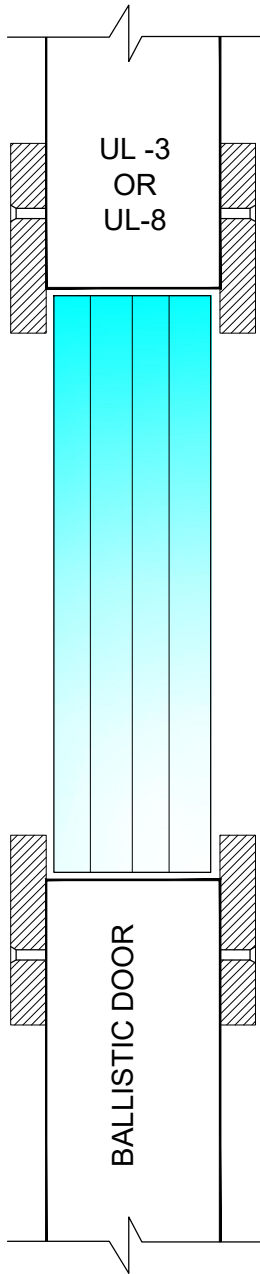
SURFACE MOUNTED BALLISTIC VISION FRAME
