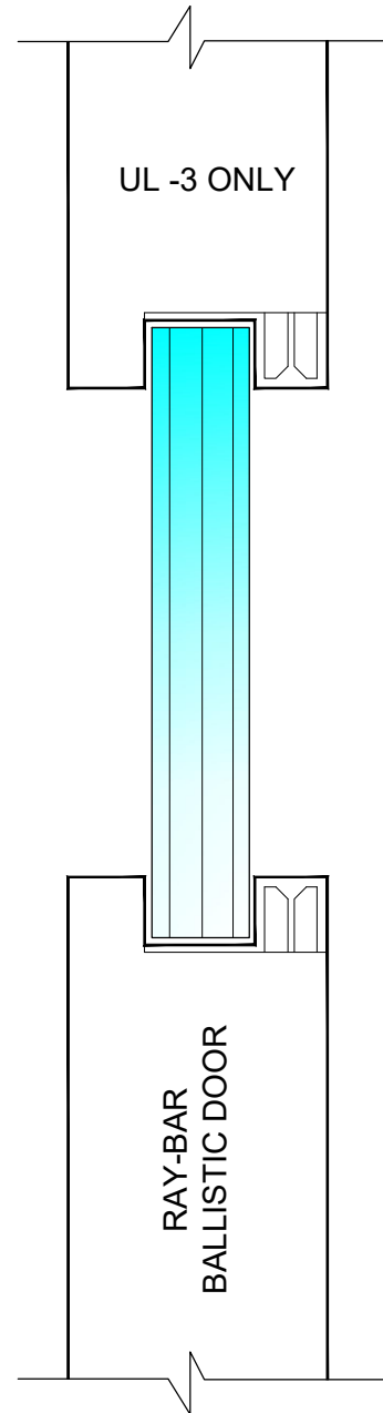
INTEGRAL - CENTERED VISION FRAME IN DOOR
