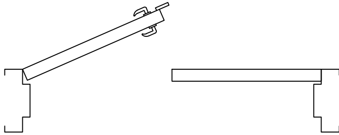
ASTRAGAL AT ACTIVE LEAF
