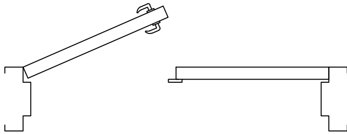
ASTRAGAL AT INACTIVE LEAF
